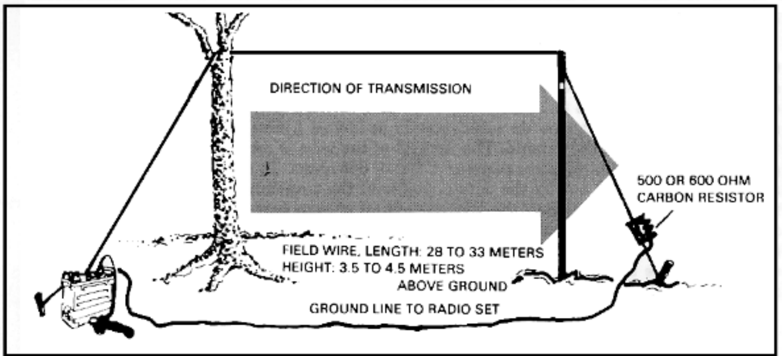
Figure 3-37. Long-wire antenna.
