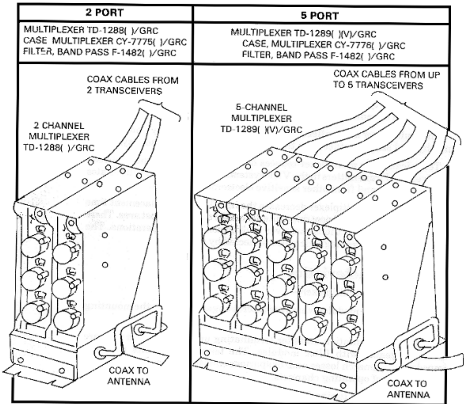
Figure D-1. Transceiver multiplexer.
