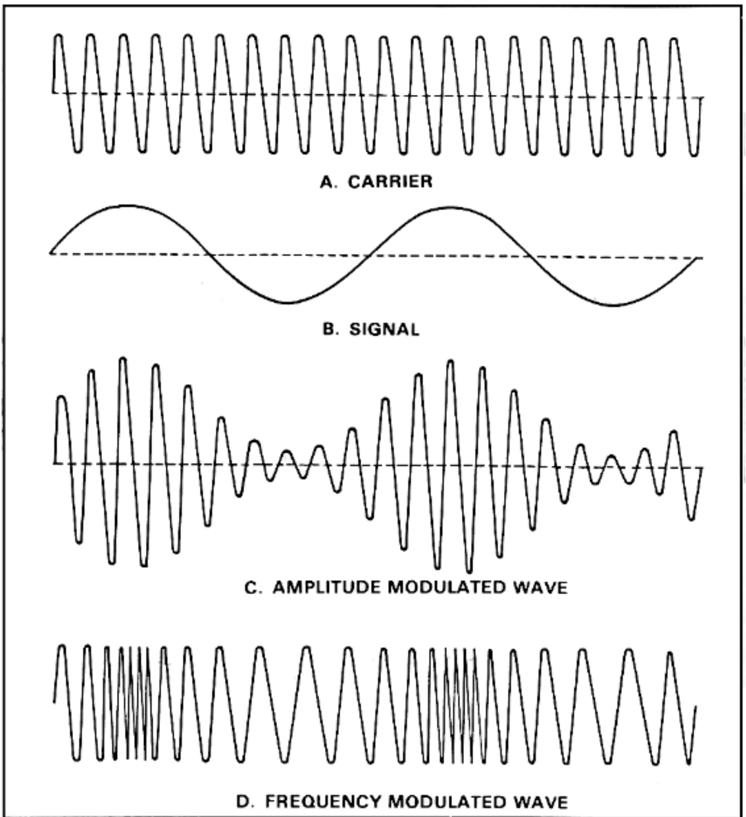
Figure 2-17. Wave shapes.
